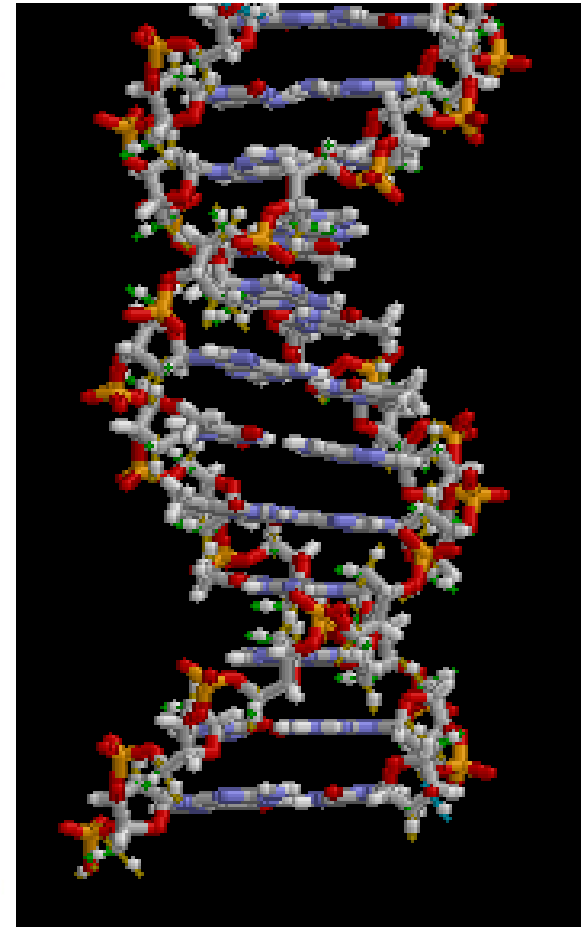
ADN
